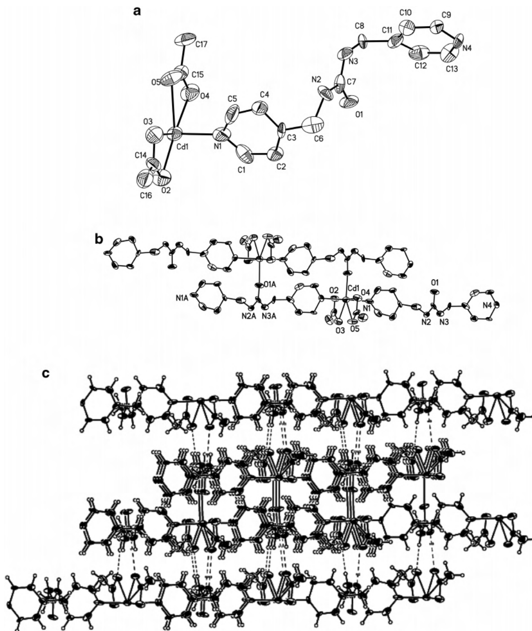
Figure 2. (a) Molecular structure (the ORTEP diagram shows 50% probability ellipsoids), (b) 1-D ladder structure, and (c) 2-D hydrogen-bonded framework of 1.
