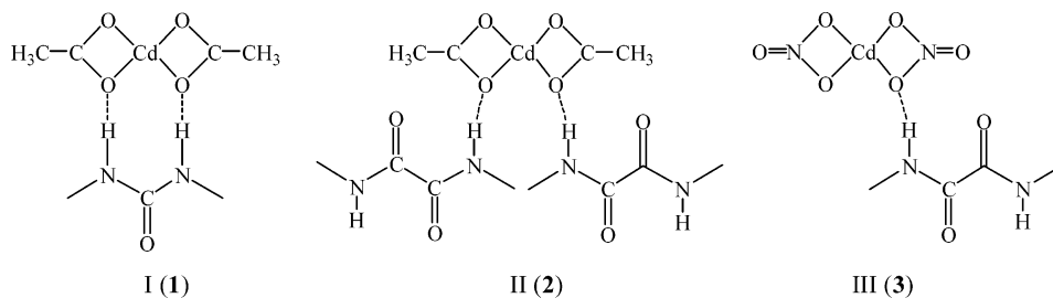
Figure 1. Three hydrogen-bonding synthons between the coordinated anions and the amide groups of 1–3.
